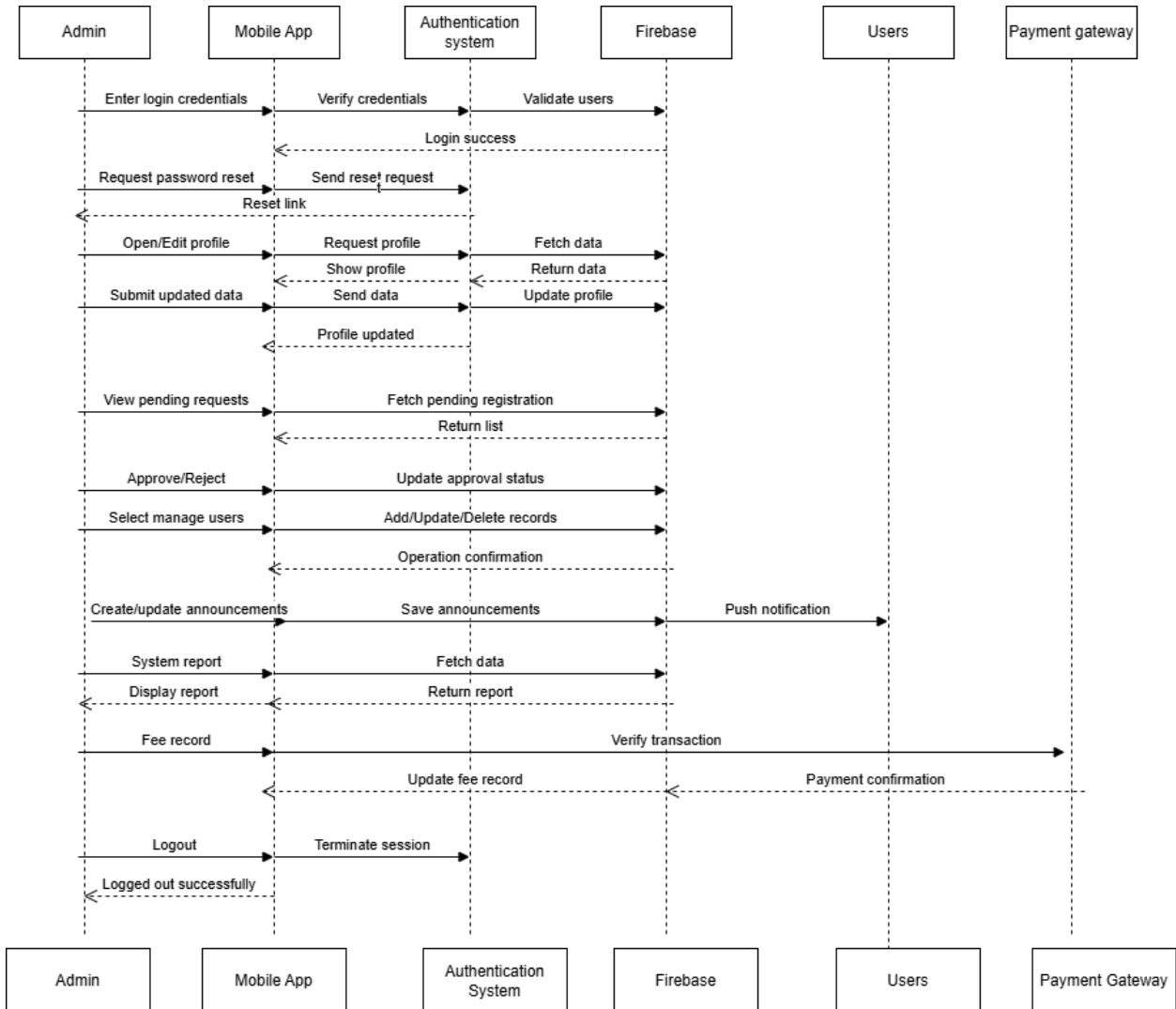
Figure 5: Sequence Diagram (Admin)
