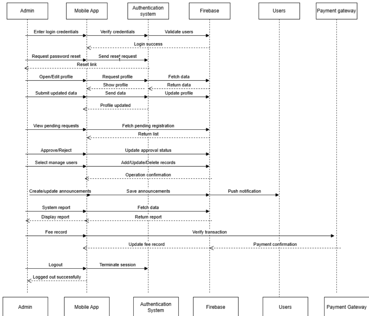
Figure 17: Sequence Diagram (Admin)
