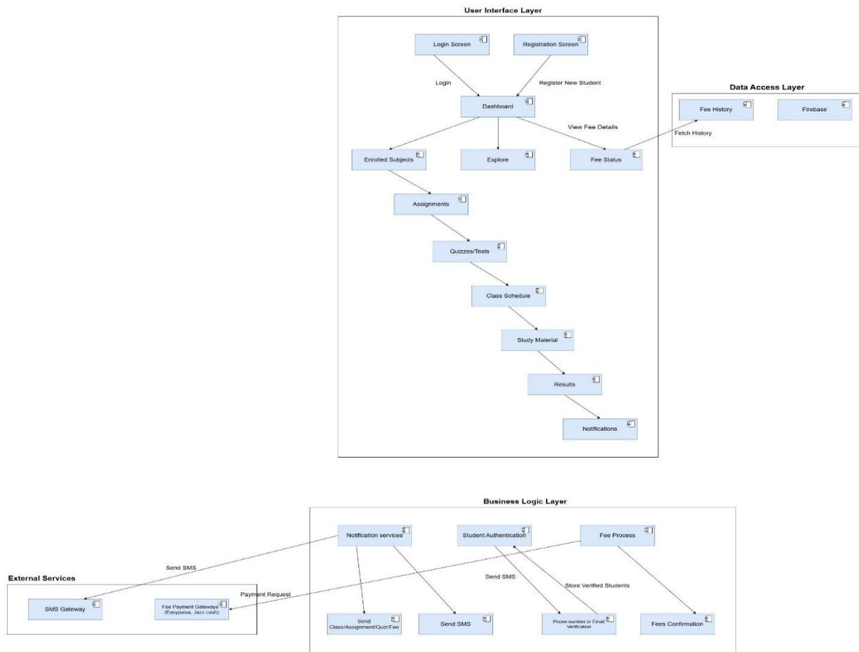
Figure 10: Architecture Diagram
